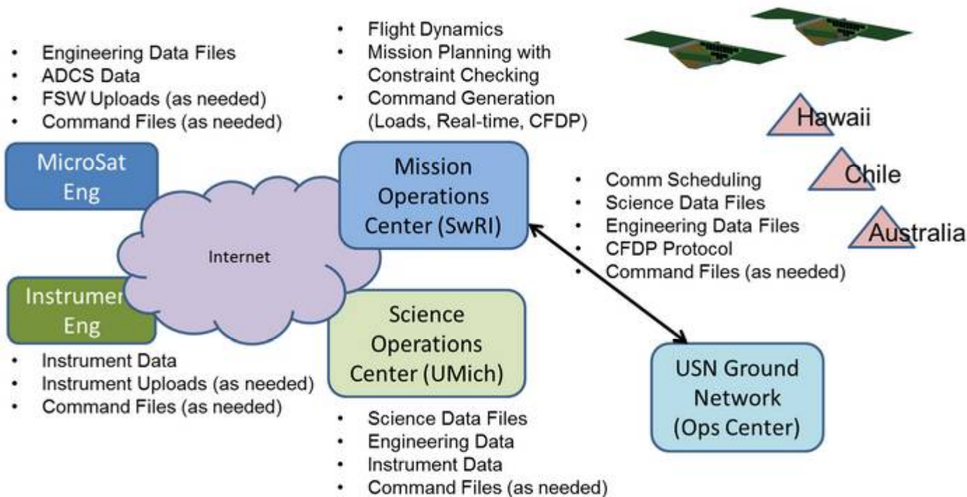
Figure 4: CYGNSS Ground System Overview
