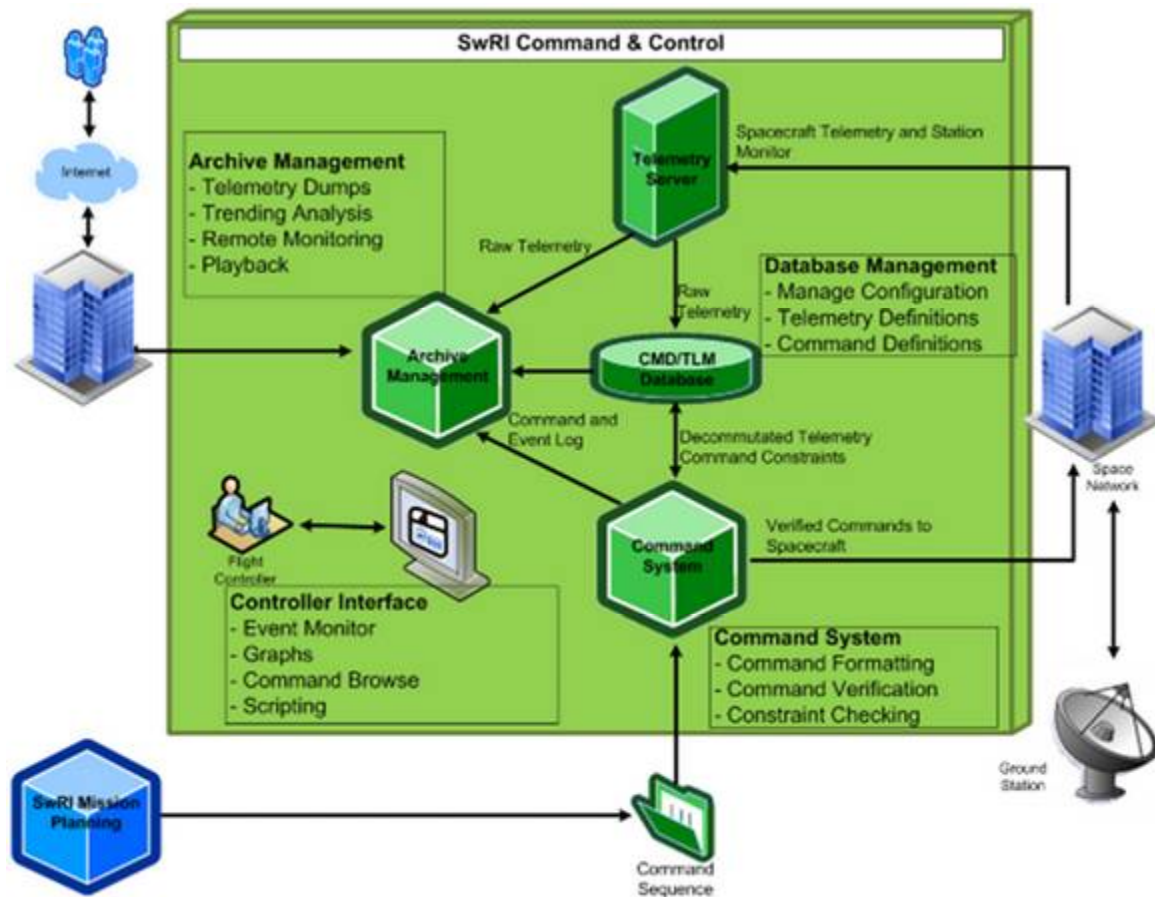
Figure 6: CYGNSS Command and Control System
