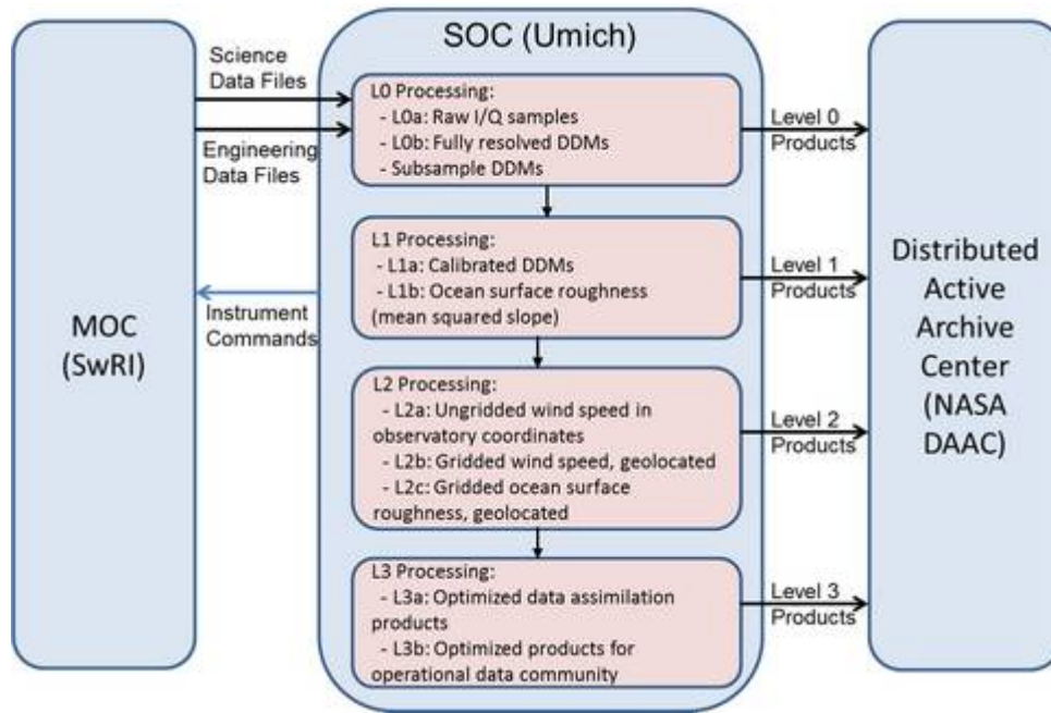
Figure 5: CYGNSS SOC Overview
