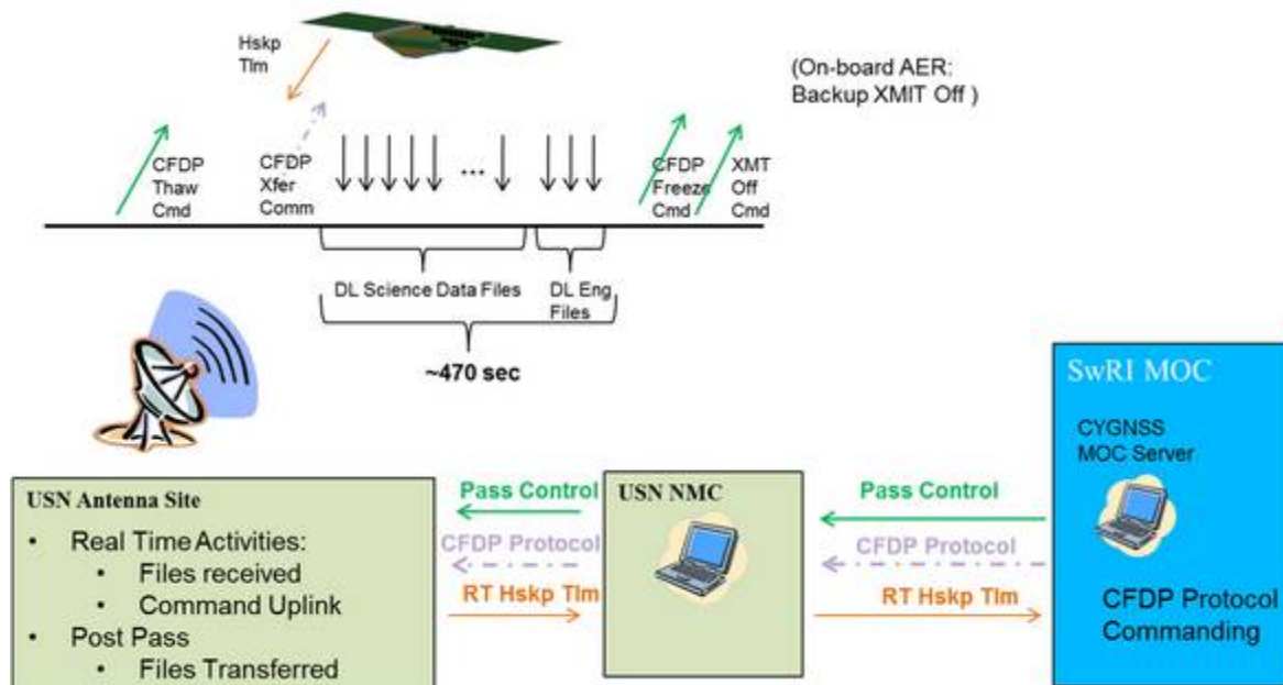
Figure 3: Communications Pass Flow
