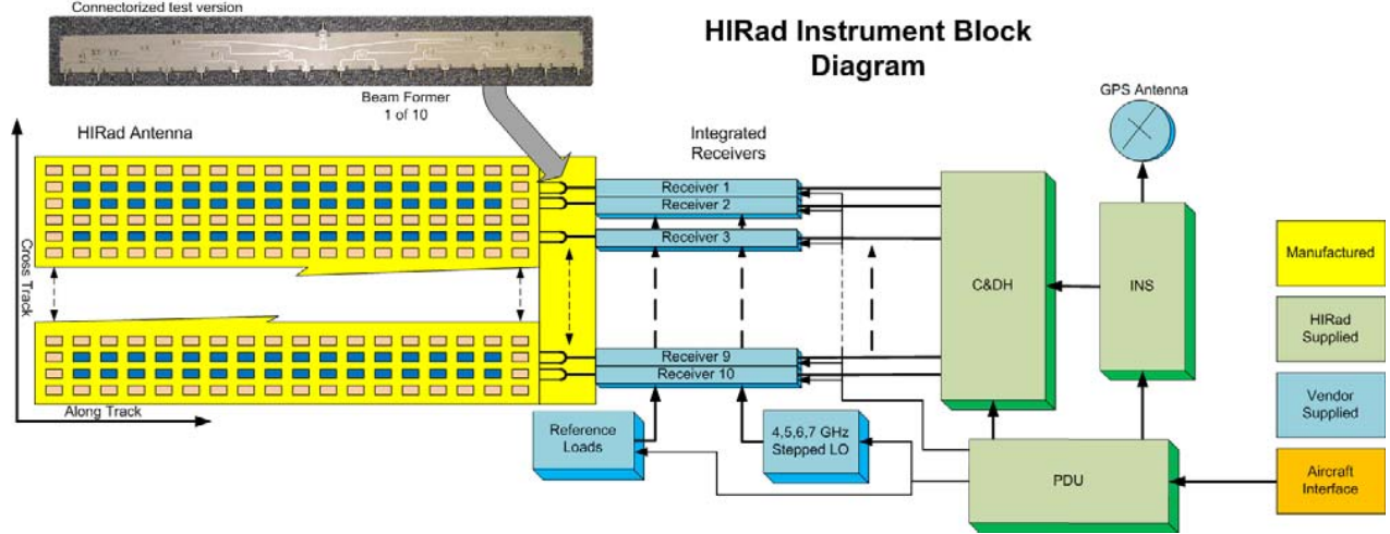
Figure 1: Radiometer System Block Diagram
