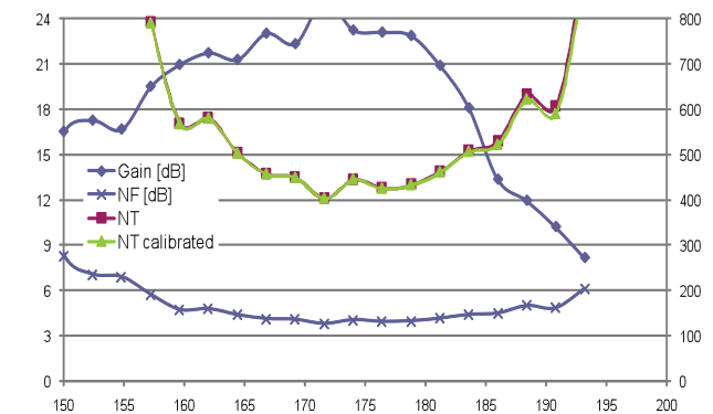
Figure 4. Gain and noise performance of receiver module.
