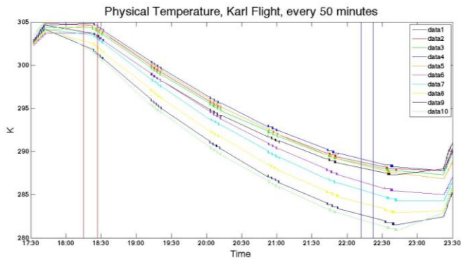
(a) Receiver temperatures during a typical flight (GRIP 2010)
