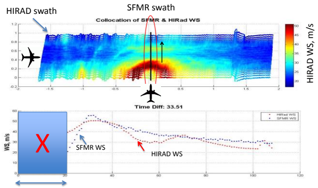
Figure 3: Comparison of HIRAD retrieved wind speed with the SFMR observed wind speed during hurricane Earl overflight.
